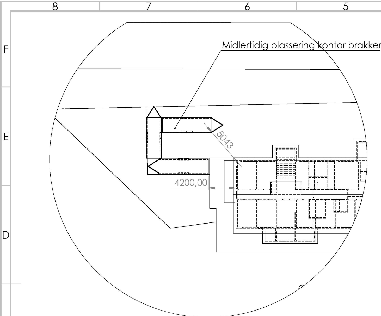
DETAIL D SCALE 1 : 300
