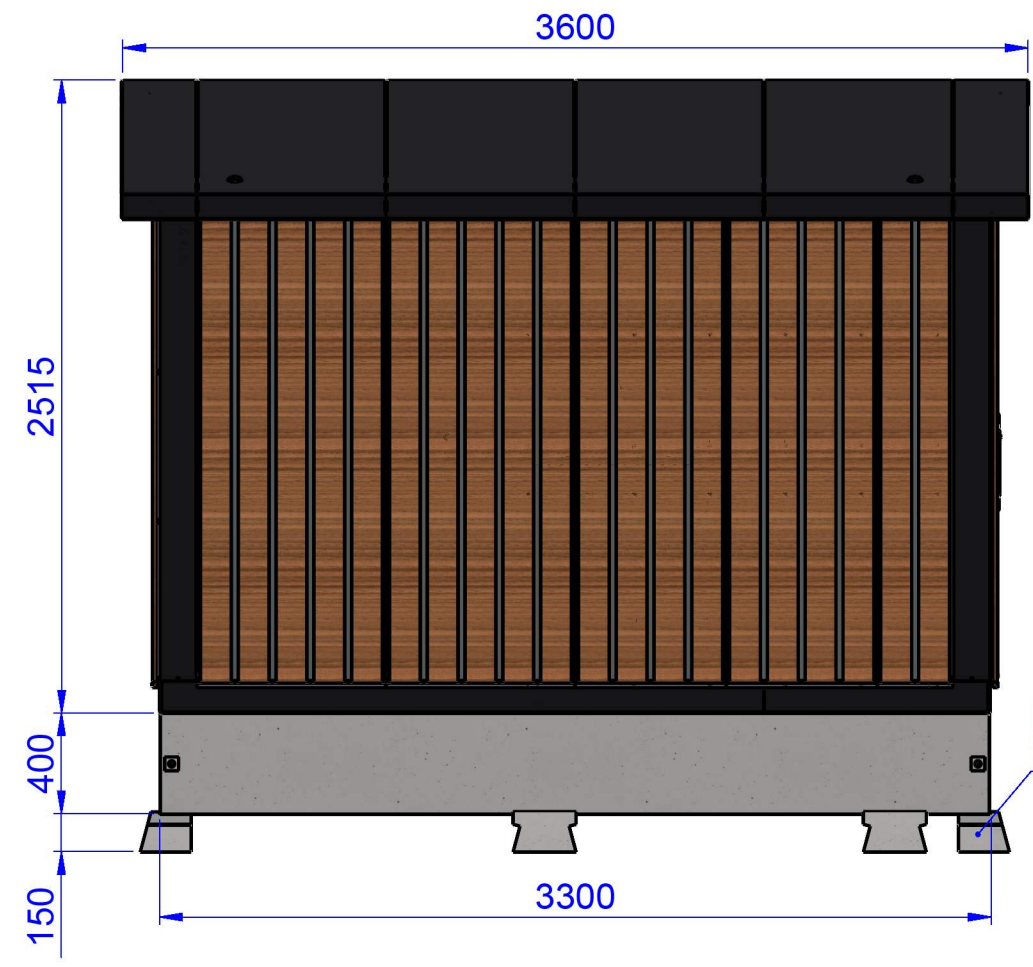
Left View
