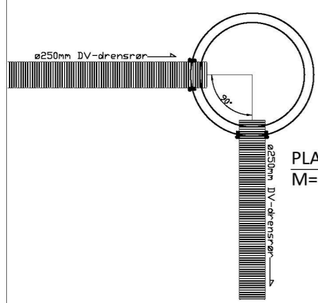
PLAN STAKE-/SANDFANGSKUM O2 M=1:50
