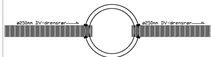
PLAN STAKE-/SANDFANGSKUM O2 M=1:50
