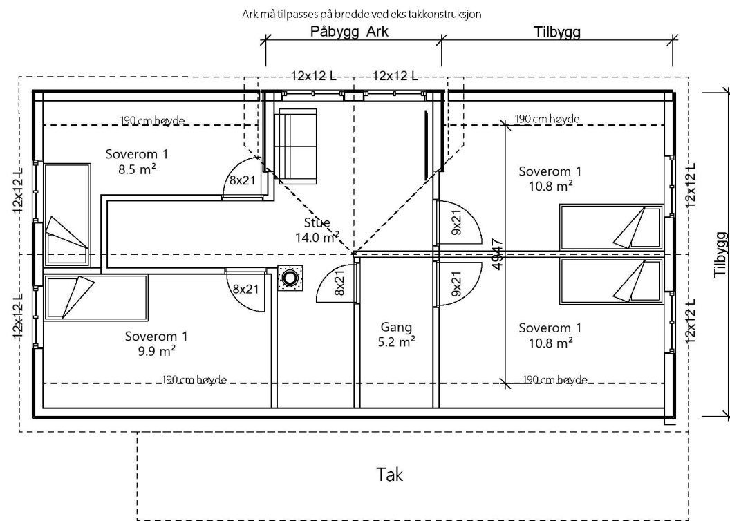
Plan 3
