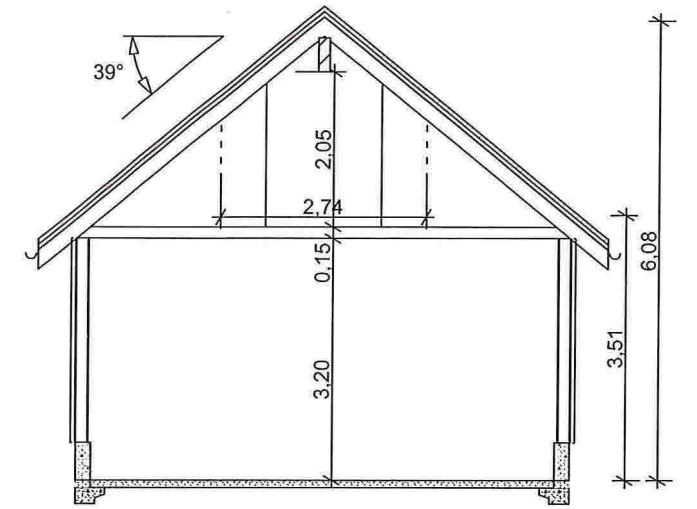
A Building Section 1:100
