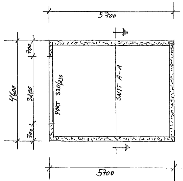
HOVED PLAN
