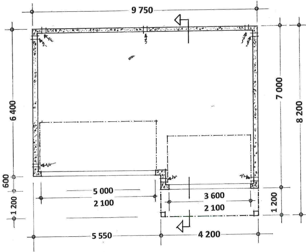
PLAN
