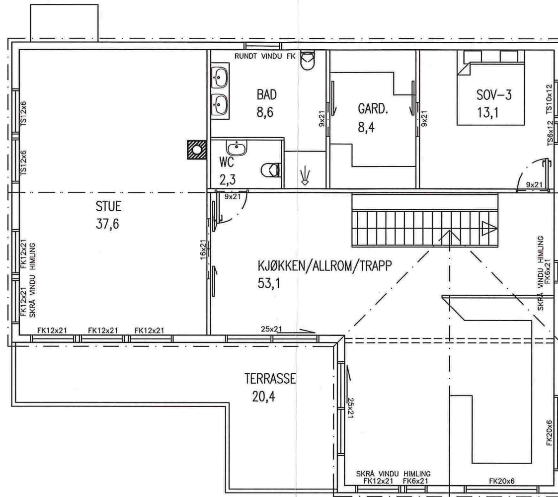
2. PLAN
