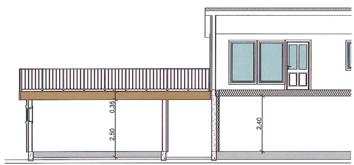
A Building Section 1:100
