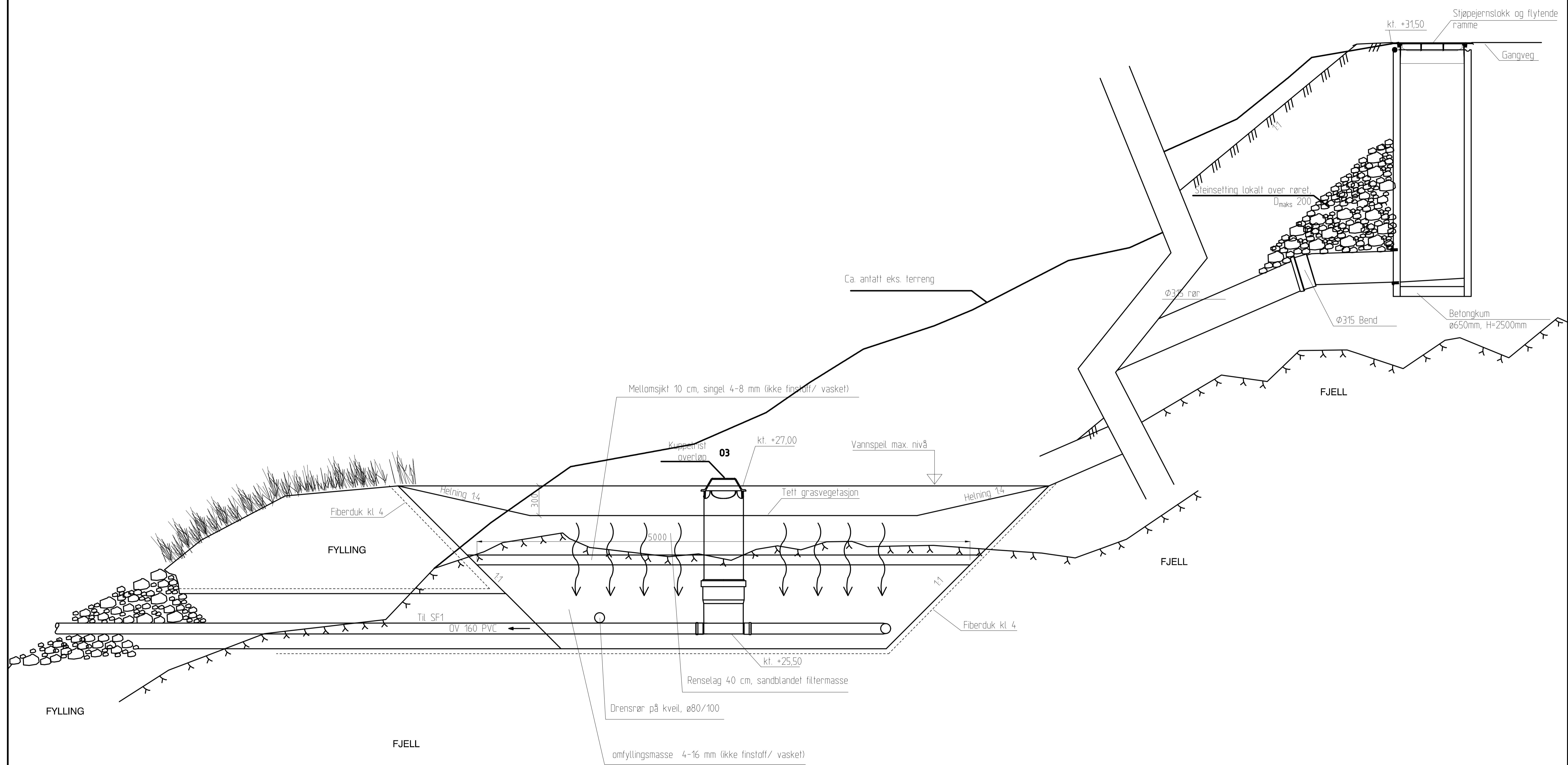
SNITT D - D RENSEFILTER M= 1:20
