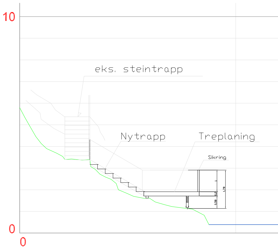
Snitt B-B Treplanning Alverparken gbnr 137/86 1-100 A4 14052020
