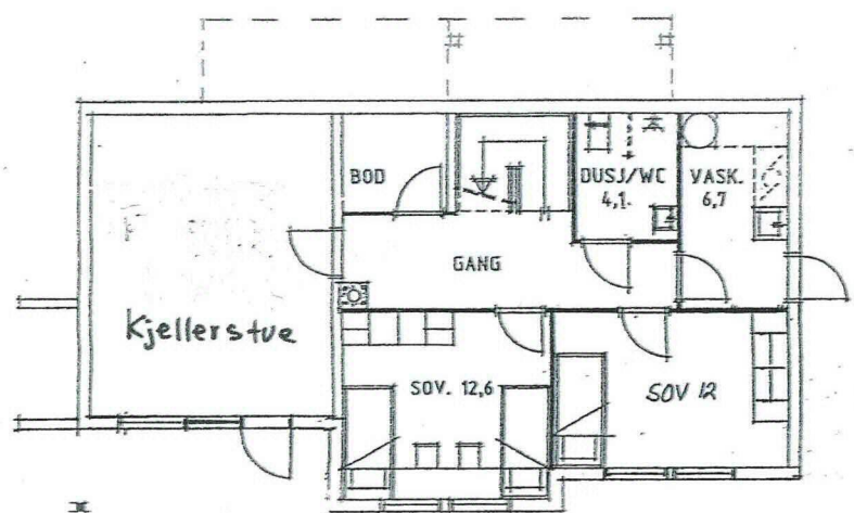
PLAN UNDER-ETG.
