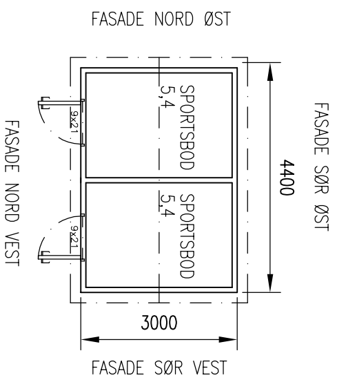
PLAN SPORTSBODER
