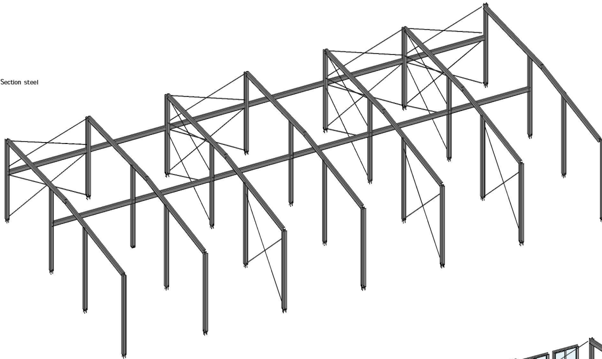
3D Section steel, windows and doors
