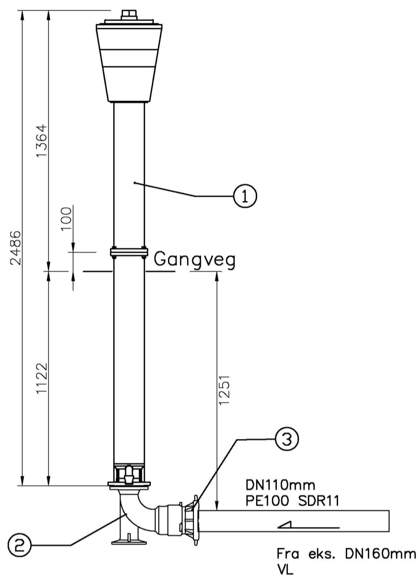
SNITT HYDRANT HY1 M=1:20
