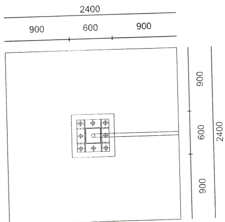
Concrete for pole 6000mm
