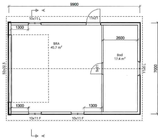
Plan BYA 70,0 m 2
