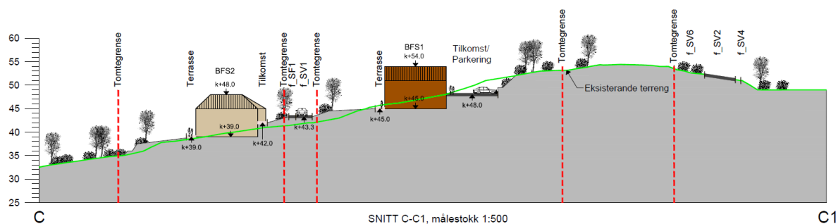
Figur 18: Snitt C-C1
