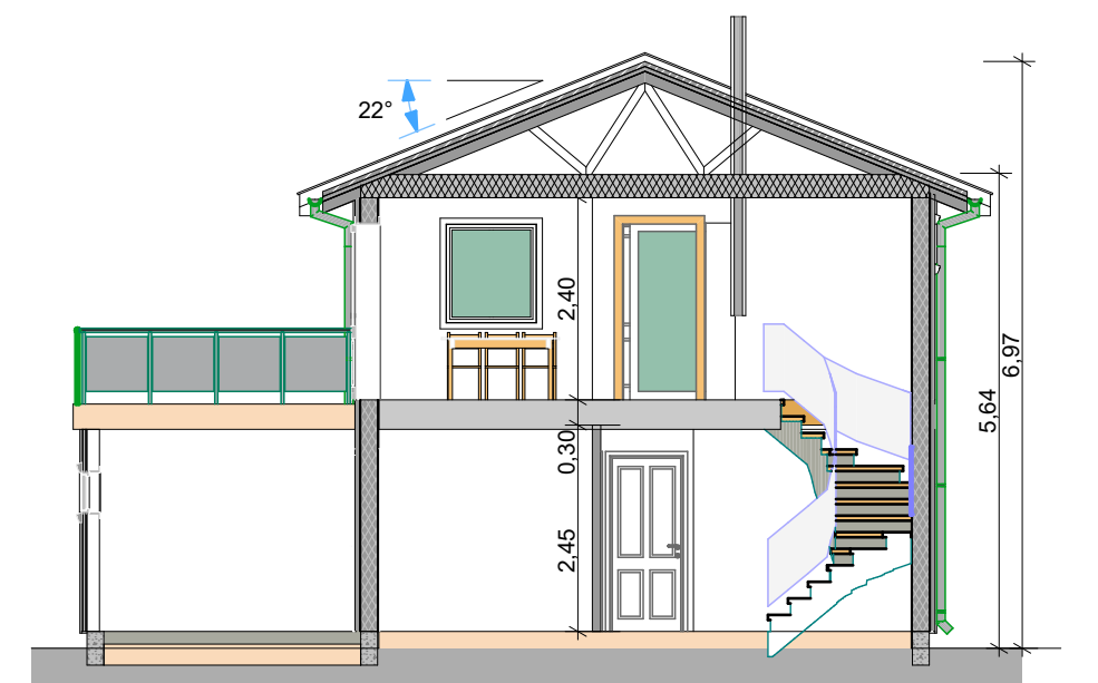
A Building Section 1:100
