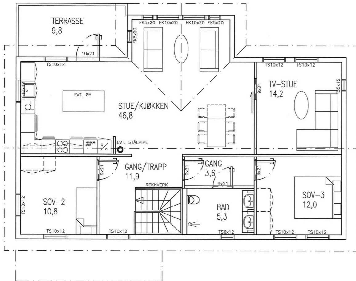
2. PLAN
