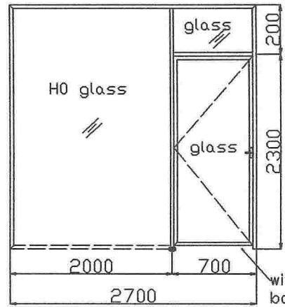
Back Wall
