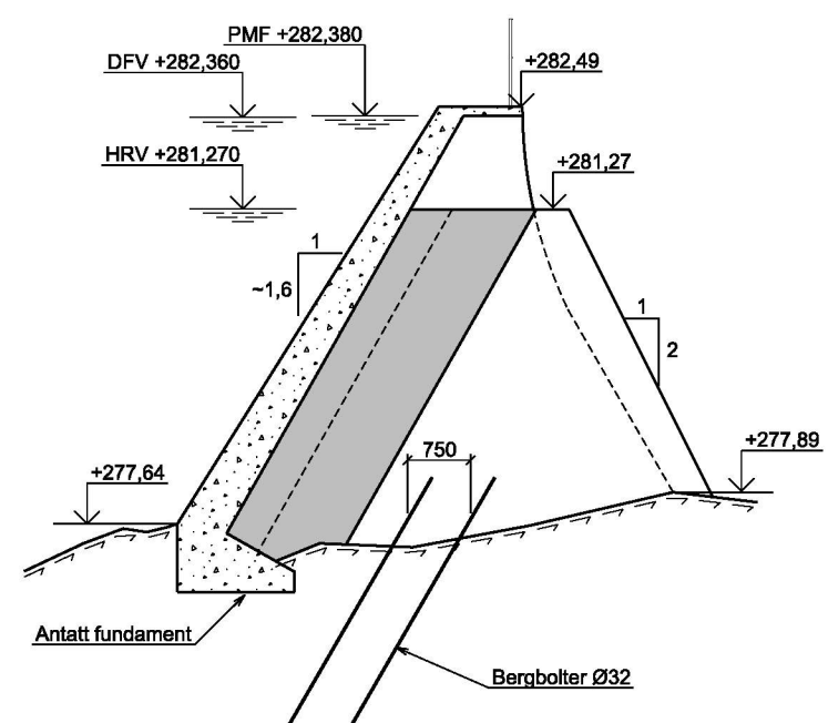
SNITT 8-8
